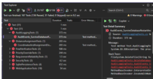
Figure 3.4.1: System.IO.IOException
